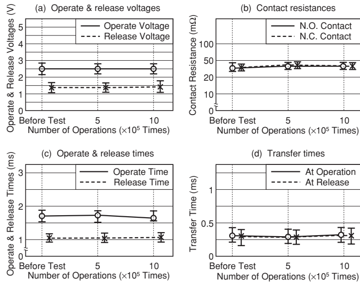
Figure 5.15 Inductive Load Test
