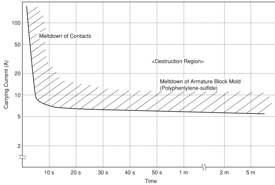
Figure 3.12 Resistance to Carrying Current
