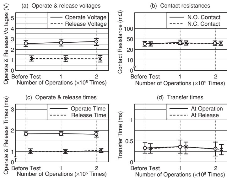
Figure 5.18 Resistive Load Test H
