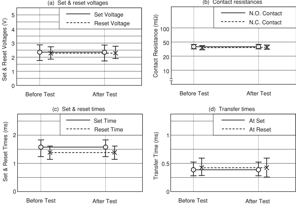
Figure 5.1 (2) High-temperature Test
