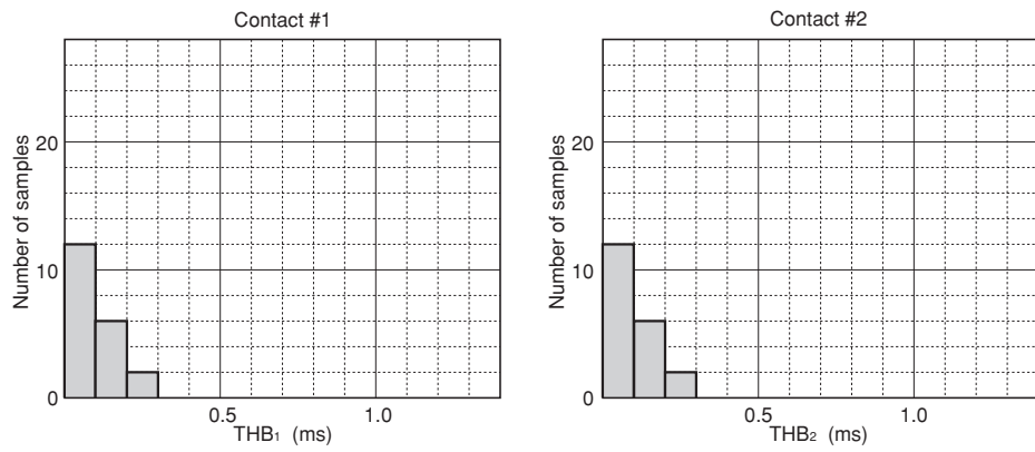
Figure 4.4C Timing
