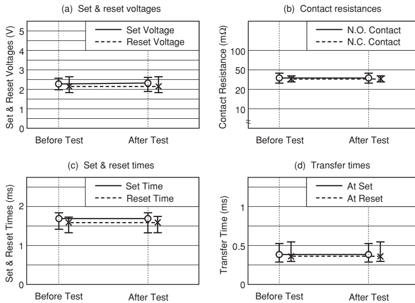
Figure 5.7 (2) Resistance to Reflow Solder Heat
