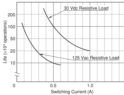
Figure 3.2 Life Curve
