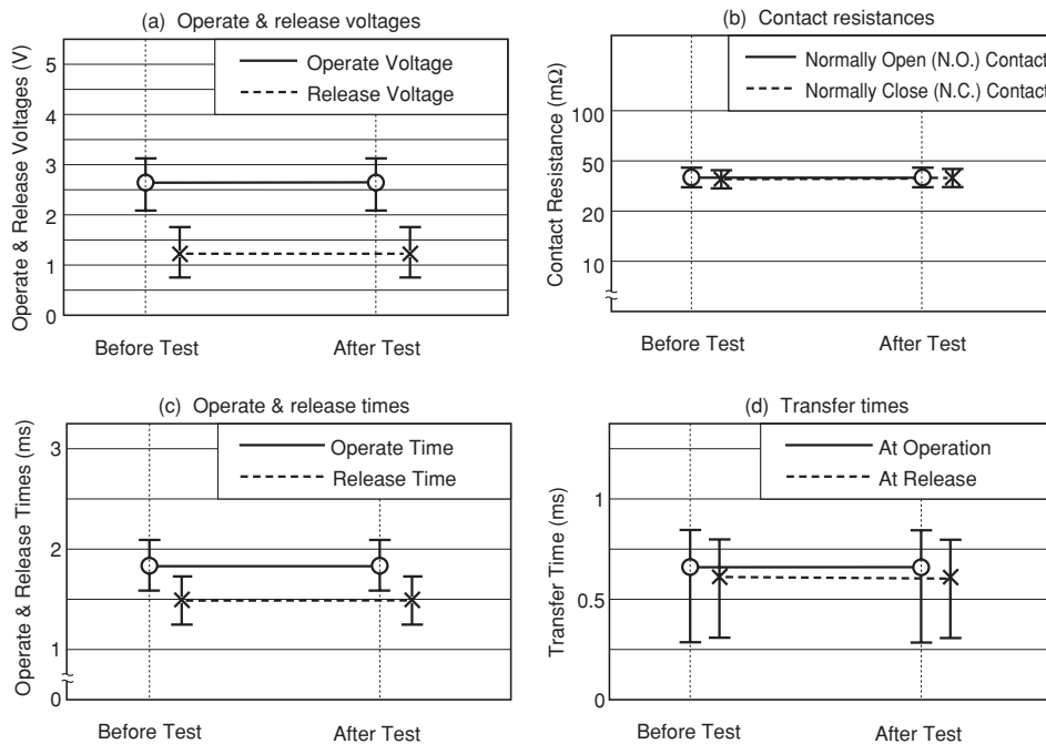
Figure 5.1 (1) High-temperature Test
