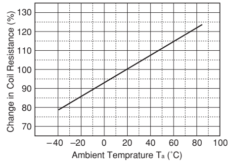
Figure 3.7 Temperature Characteristics
