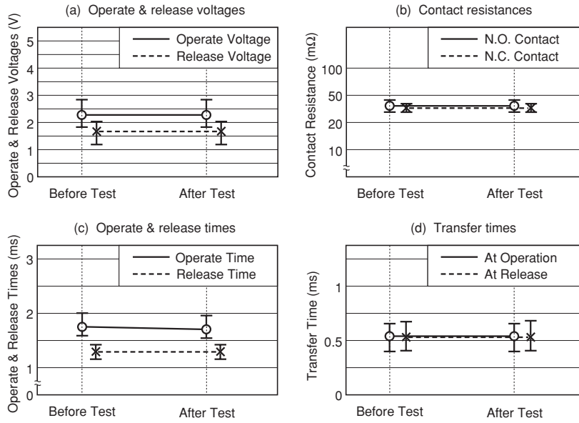
Figure 5.7 (1) Resistance to Reflow Solder Heat
