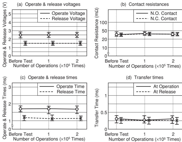
Figure 5.17 Resistive Load Test G
