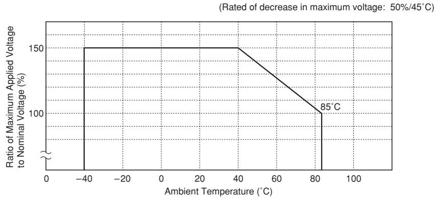
Figure 3.3 Maximum Voltage Applied to Coil
