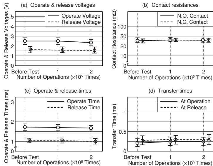
Figure 5.16 Resistive Load Test F
