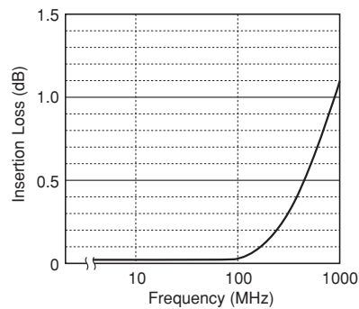
Figure 3.9 High-frequency characteristics
