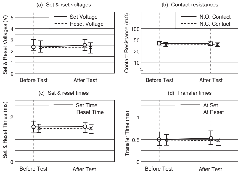
Figure 5.5 (2) Vibration Test
