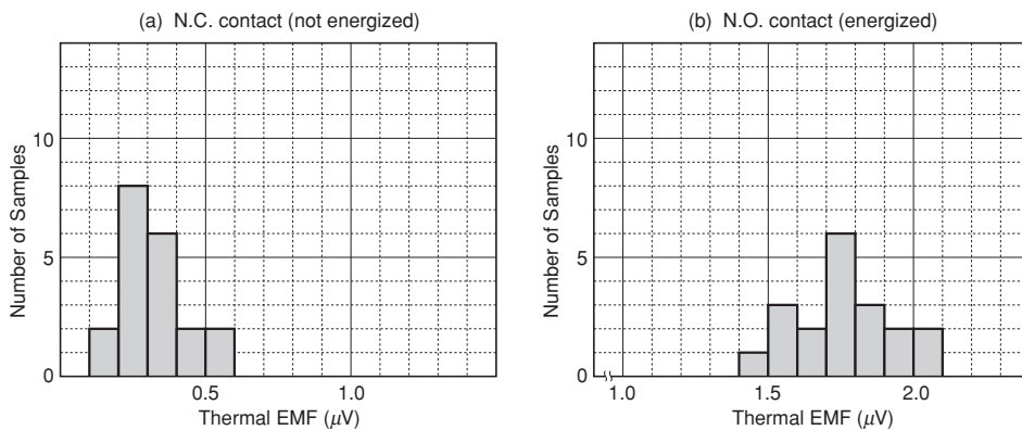
Figure 4.7 Thermal EMF
