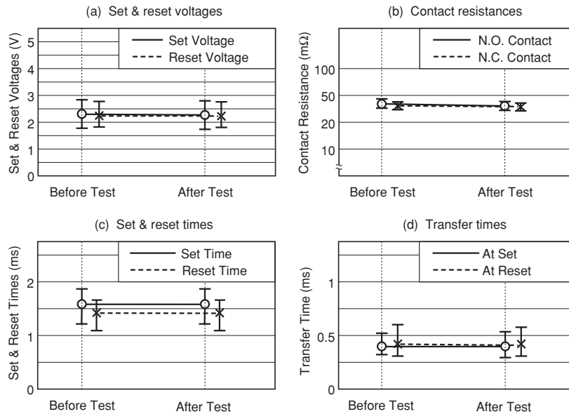
Figure 5.2 (2) Low-temperature Test
