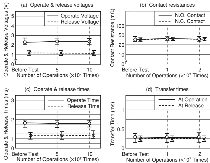
Figure 5.9 Non-load Test B
