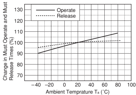
Figure 3.7 Temperature Characteristics
