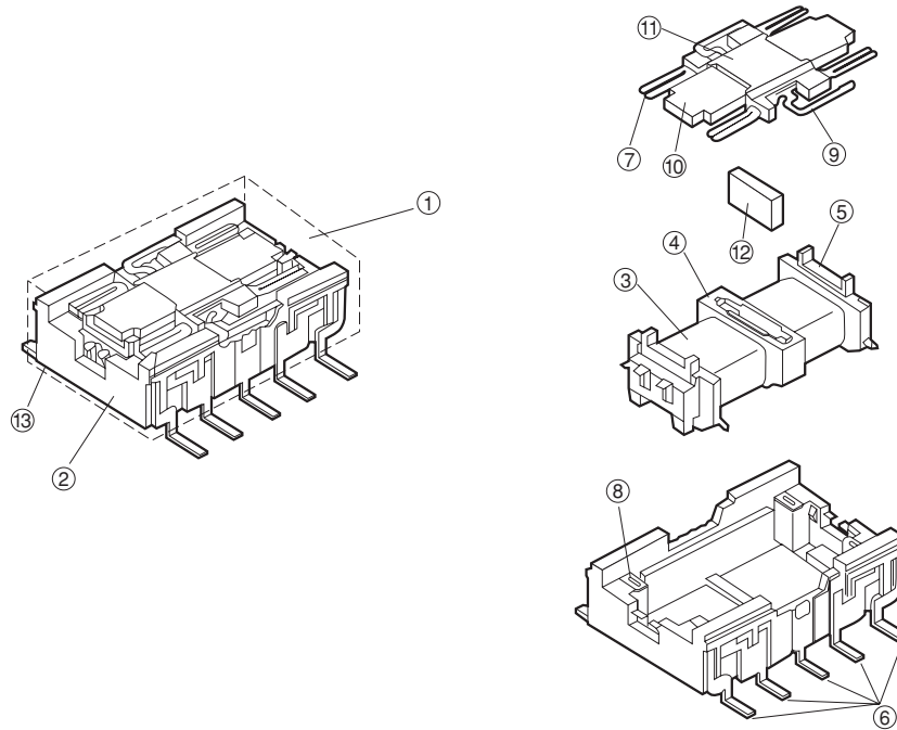
Figure 2.1 Structure of the EB2 Series Relay
