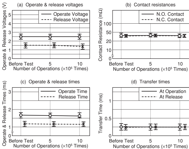
Figure 5.14 Resistive Load Test E
