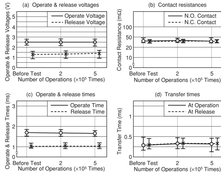
Figure 5.12 Resistive Load Test C
