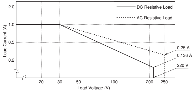
Figure 3.1 Switching Power
