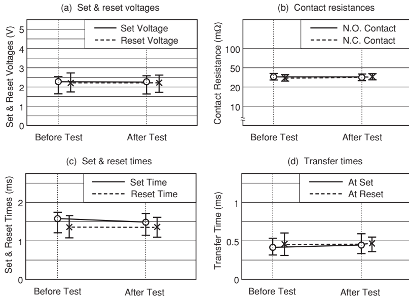
Figure 5.6 (2) Shock Test
