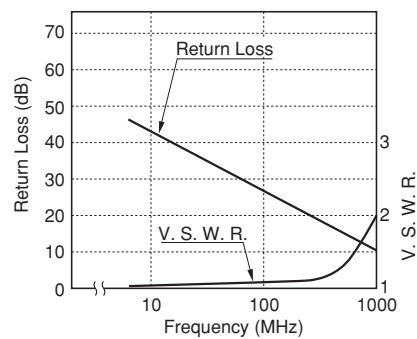
Figure 3.9 High-frequency characteristics
