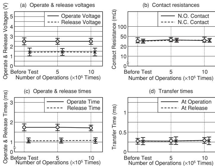
Figure 5.13 Resistive Load Test D
