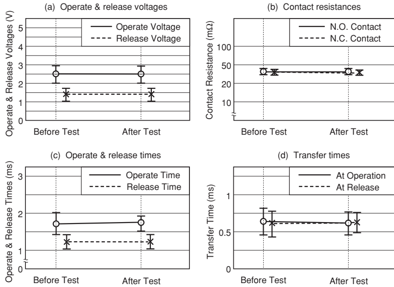
Figure 5.6 (1) Shock Test
