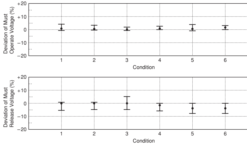
Figure 3.8 Magnetic Interference
