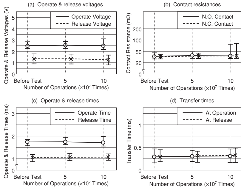
Figure 5.8 Non-load Test A
