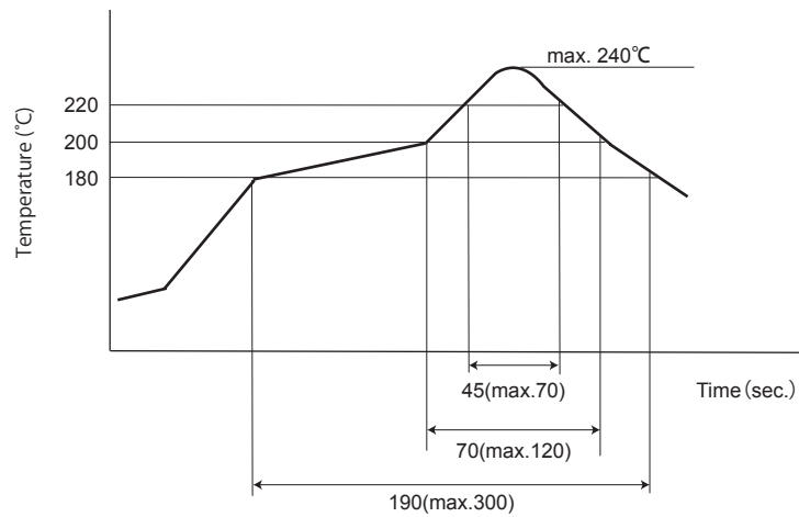
Figure 5.7 Temperature Profiles
