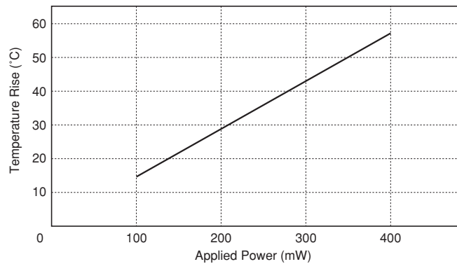
Figure 3.4 Coil Temperature Rise
