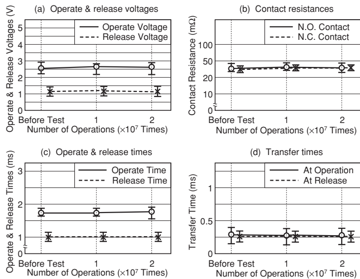
Figure 5.10 Resistive Load Test A
