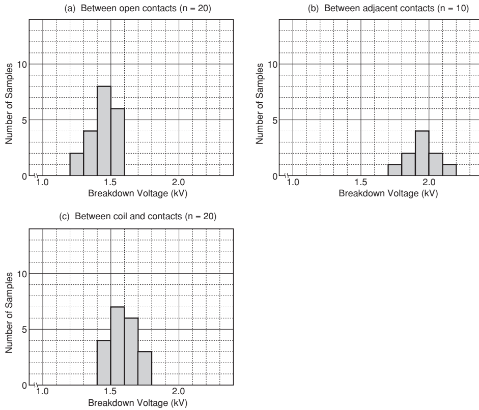
Figure 4.6 Breakdown Voltage
