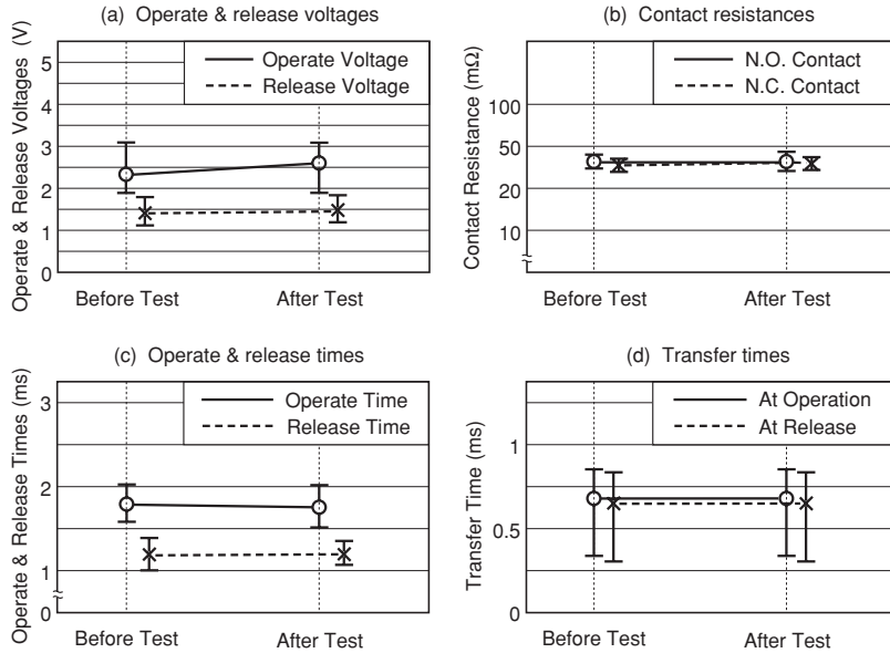
Figure 5.5 (1) Vibration Test
