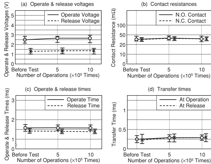
Figure 5.11 Resistive Load Test B
